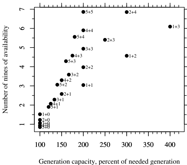
FIGURE 14.19 Theoretical availability with different generation configurations. The graph assumes an individual unit is 97% available. The k + n notation means k generators are needed to meet the peak load, and the site has n extra generators. (Copyright © 2002. Electric Power Research Institute. 1007281. Analysis of Extremely Reliable Power Delivery Systems . Reprinted with permission.)
