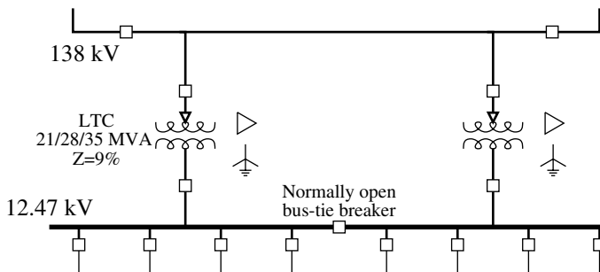
FIGURE 1.13 Example suburban distribution substation.
