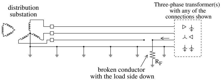
FIGURE 4.31 Backfeed to a downed conductor.
