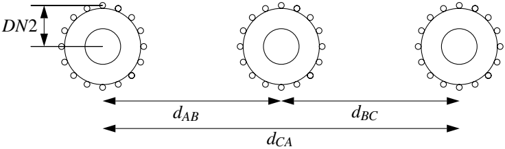
FIGURE 3.6 Cable dimensions for calculating impedances.
